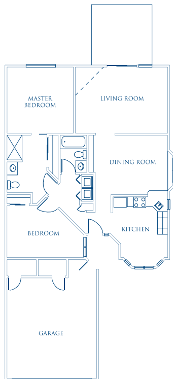
Cottage Floor Plan: Approx 1,300 SF
